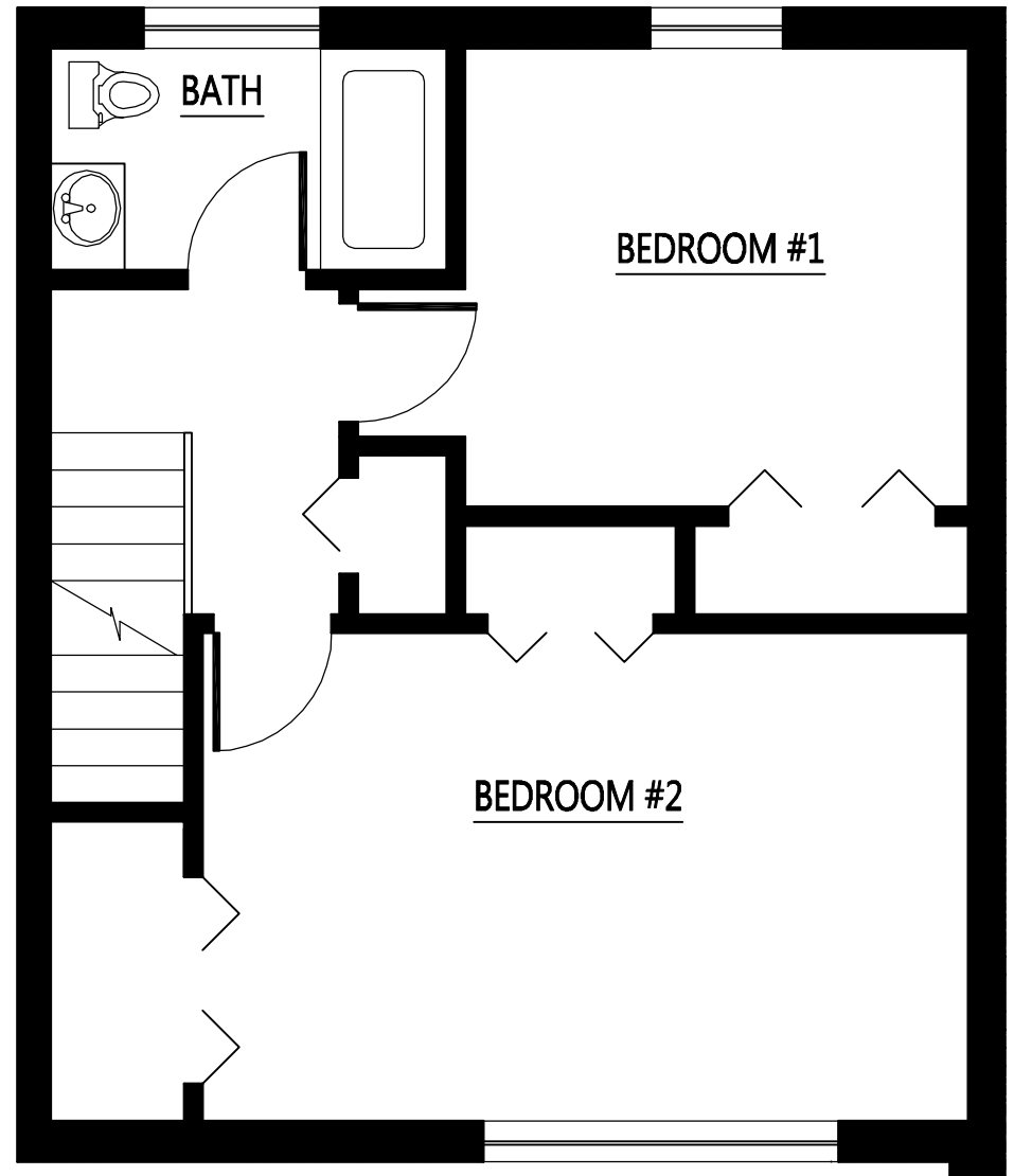
UPPER PLAN AREA = 475 SQFT
